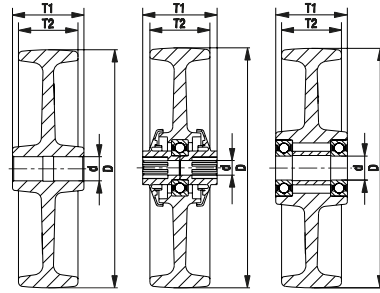
plain bore ball bearing (C) KA version ball bearing
